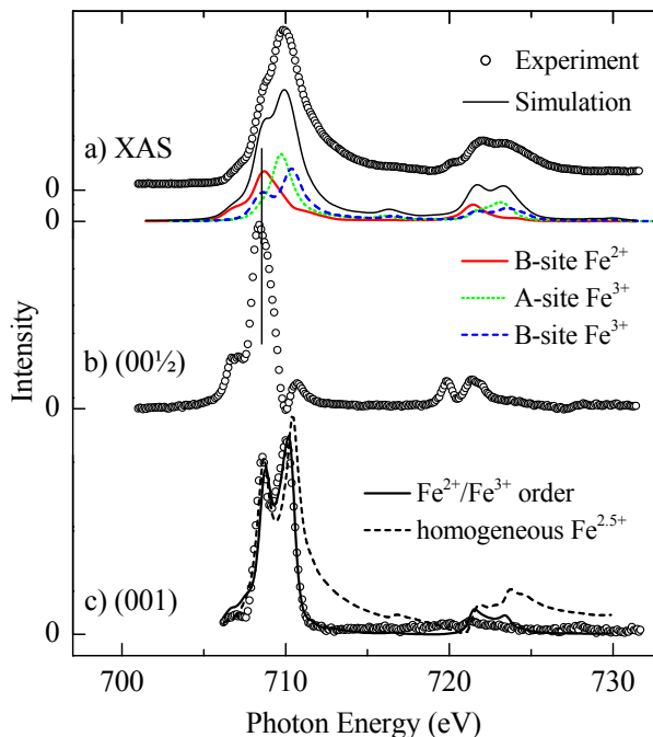
FIG. 3: (color online). a) Experimental Fe L_{2,3} XAS spectra of \text{Fe}_3\text{O}_4 (symbols). The black thin solid line is a simulation, which is constructed as the sum of the spectra from the B-site \text{Fe}^{2+} (red thick solid line), A-site \text{Fe}^{3+} (green dotted line), and B-site \text{Fe}^{3+} (blue dashed line) ions; b) energy dependence of the (001/2) diffraction peak intensity; c) energy dependence of the (001) intensity (symbols), the solid line is a simulation for a charge-order scenario and the dashed line for a homogeneously mixed-valent scenario, both scaled to the height of the first resonance peak.
