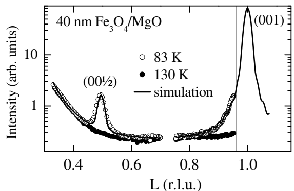
FIG. 1: Scan along L below (open symbols) and above (filled symbols) T_V recorded at 708.5 eV photon energy with \sigma polarization. The solid line through the data points is a simulation. The vertical line at L=0.96 denotes the maximum possible momentum transfer at this energy.
