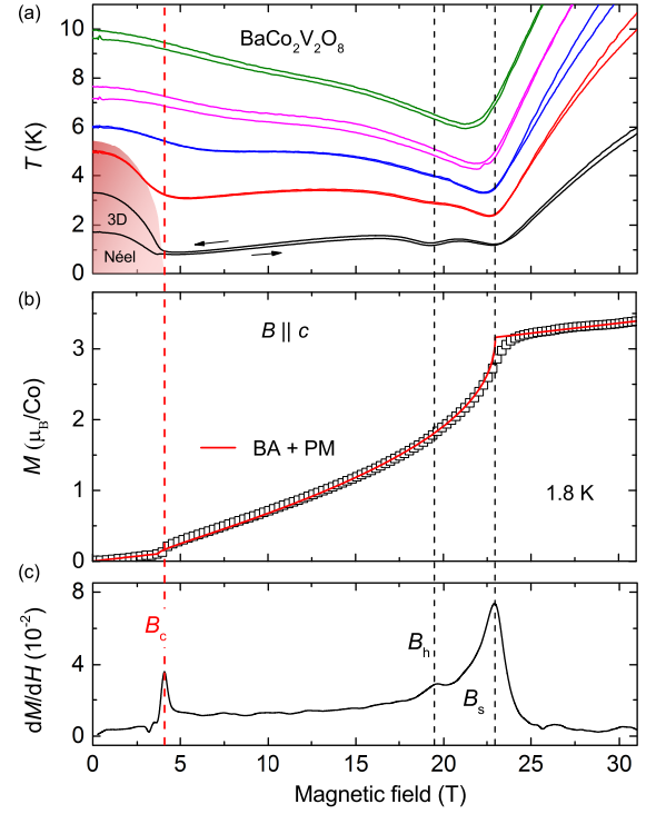
Figure 2. (a) Magnetocaloric-effect T(B) , (b) magnetization M(B) , and (c) differential susceptibility dM/dH measured as a function of longitudinal field B \parallel c . The critical field B_c = 3.8 T, and the characteristic fields B_h = 19.5 and B_s = 22.9 T corresponding to half-saturated and saturated magnetizations, respectively, yield minima of T(B) and peaks of dM/dH at the lowest temperature, as marked by the dashed lines. In (a), the shaded area indicates the 3D Néel ordered phase [43]. In (b), the solid line is obtained from Bethe Ansatz (BA) solution of the Heisenberg-Ising model, in addition to a paramagnetic (PM) background.
