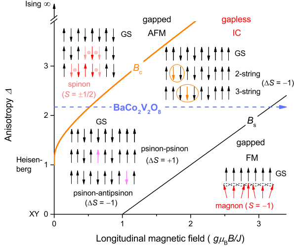
Figure 1. Phase diagram of the antiferromagnetic XXZ spin-1/2 chain with the anisotropy parameter \Delta in a longitudinal magnetic field. The different regimes (gapped or gapless) are separated by the critical field B_c and saturation field B_s , and are characterized by distinct ground states (GS) and characteristic excitations (magnons, spinons, psinons, antipsinons, and strings) due to a "spin flip", as schematically illustrated by the insets. The dashed line indicates an increasing magnetic field at \Delta = 2.17 for \text{BaCo}_2\text{V}_2\text{O}_8 .
