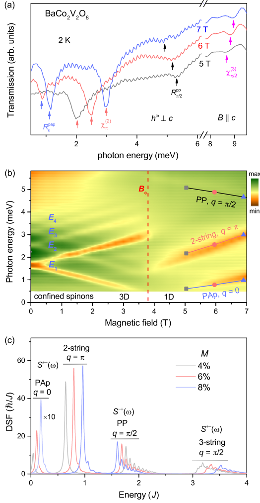
Figure 4. (a) Transmission spectra for the polarization \hbar\omega \perp c obtained at 2 K in the longitudinal fields above B_c . Excitations of 2-strings \chi_{\pi/2}^{(2)} , 3-strings \chi_{\pi/2}^{(3)} , psinon-antipsinon R_0^{pap} pairs, and psinon-psinon R_{\pi/2}^{pp} pairs are indicated, as identified by comparing to Bethe Ansatz results. The weak wiggly-like feature is due to multiple interference within the sample. (b) Contour plot of transmission at 2 K. For B < B_c , confined-spinon levels E_i are observed. For B > B_c , different excitations with distinct slopes are observed, as for the string and fractional excitations. (c) Dynamic structure factors (DSF) S^{+-} and S^{-+} obtained via Bethe Ansatz for the magnetizations 2, 4, 6% of the saturated value. For clarity, the DSF for PAp is multiplied by a factor of 10.
