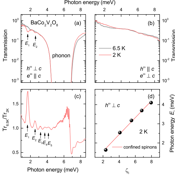
Figure 3. Transmission spectra measured at 6.5 and 2 K, above and below T_N \simeq 5.5 K, respectively, for the polarizations (a) h^\omega \perp c , e^\omega \parallel c and (b) h^\omega \parallel c , e^\omega \perp c . (c) The ratio of the transmission spectra at 6.5 and 2 K from (a) reveals absorption peaks, as indicated by the arrows, which signal the excitations of confined spinons below T_N . (d) The energy hierarchy of these excitations linearly depends on \zeta_i , as expected for confined spinons in a linear confining potential [34].
