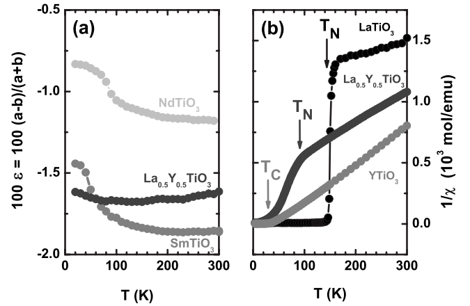
FIG. 9. (a) Orthorhombic splitting \varepsilon of La_{1-x}Y_xTiO_3 ( x=0.50 ) compared with the other RTiO_3 with similar rare-earth ionic radii. (b) Inverse magnetic susceptibility 1/\chi of La_{0.5}Y_{0.5}TiO_3 compared with those in LaTiO_3 and in YTiO_3 .
