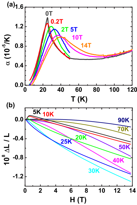
FIG. 6. (Color online) (a) Thermal expansion \alpha = 1/l \partial l / \partial T of \text{YTiO}_3 for various magnetic fields as a function of temperature ( H \parallel a ). (b) Magnetostriction \Delta L(H)/L of \text{YTiO}_3 as a function of applied magnetic field H \parallel a .
