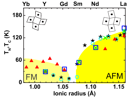
FIG. 7. (Color online) Magnetic phase diagram for \text{RTiO}_3 and \text{La}_{1-x}\text{Y}_x\text{TiO}_3 . T_C and T_N are plotted as a function of the rare-earth ionic radius. Squares: T_C , T_N for \text{RTiO}_3 from this work. Triangles: values for \text{RTiO}_3 from Greedan (Ref. 33). Crosses: values for \text{RTiO}_3 from Katsufuji et al. (Ref. 55). Circles: values for \text{La}_{1-x}\text{Y}_x\text{TiO}_3 from Okimoto et al. (Ref. 3). Stars: values for \text{La}_{1-x}\text{Y}_x\text{TiO}_3 from Goral et al. (Ref. 56). The insets show the principal octahedral deformations of the end members.
