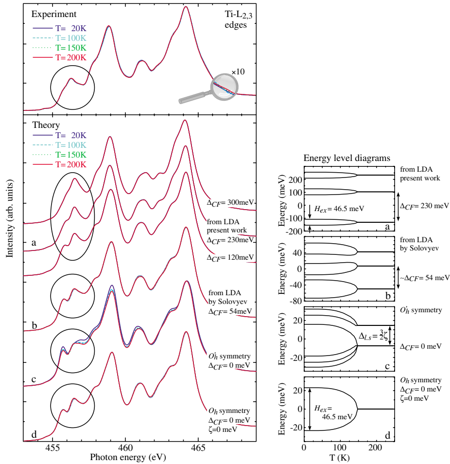
FIG. 3 (color online). Top panel: experimental Ti L_{2,3} XAS spectra taken from a twinned LaTiO 3 single crystal at 20, 100, 150, and 200 K. Left panel: simulated isotropic spectra calculated for a TiO 6 cluster at 20, 100, 150, and 200 K for several CF parameters. Right panel: corresponding energy level diagrams for the cluster in an exchange field of H_{ex} = 46.5 meV (from Keimer et al. [7]) at T = 0 K and vanishing at T_N = 146 K. Four scenarios are presented: (a) noncubic symmetry with \Delta_{CF} = 230 meV from our LDA calculation [19] and with \Delta_{CF} = 120 and 300 meV, (b) noncubic symmetry with \Delta_{CF} = 54 meV from Solovyev [11], (c) O'_h , and (d) O_h symmetry. The spin-orbit constant \zeta is 15.2 meV for (a), (b), and (c), and 0 for (d). Note the very different energy scales.
